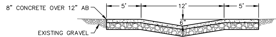
C ACCESS ROAD CROSSING N.T.S.
